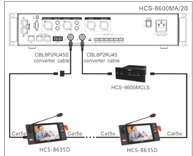
Figure 3.4.5 “Closed Loop - Daisy Chain” connection between the CMU and HCS-8635 series compact multimedia terminals
