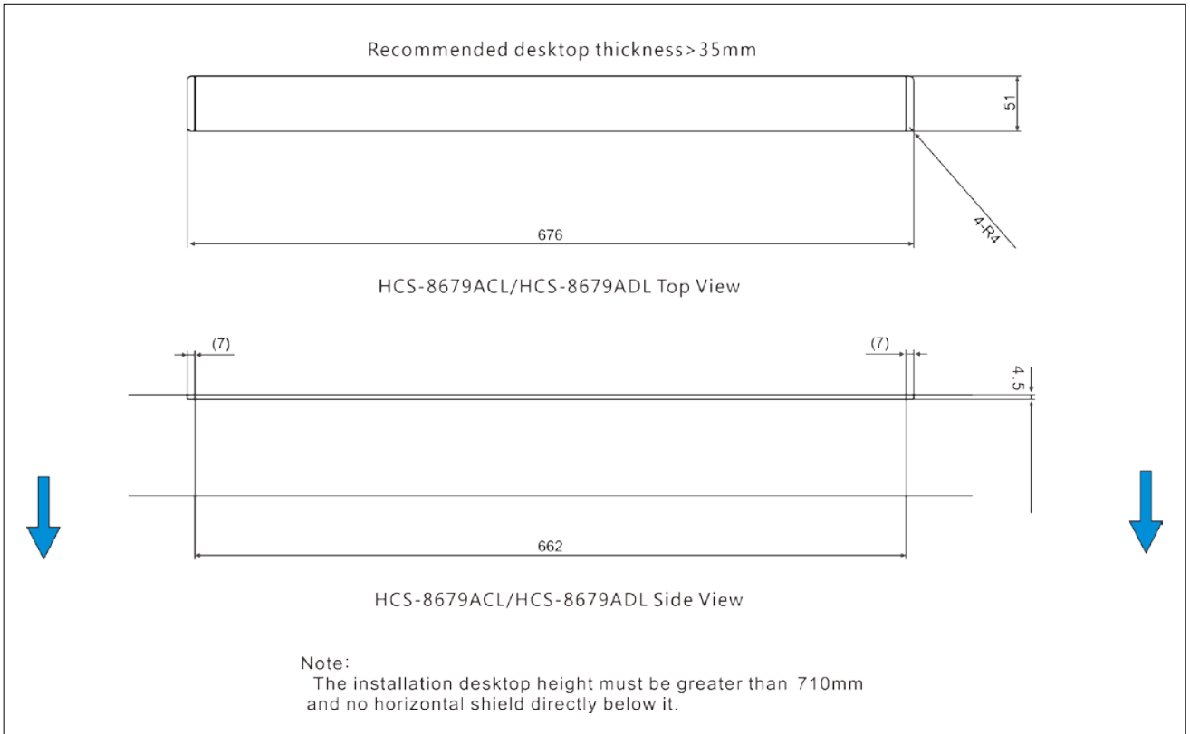
Figure: 3.2.6 Fixed installation of HCS-8679 series congress unit
