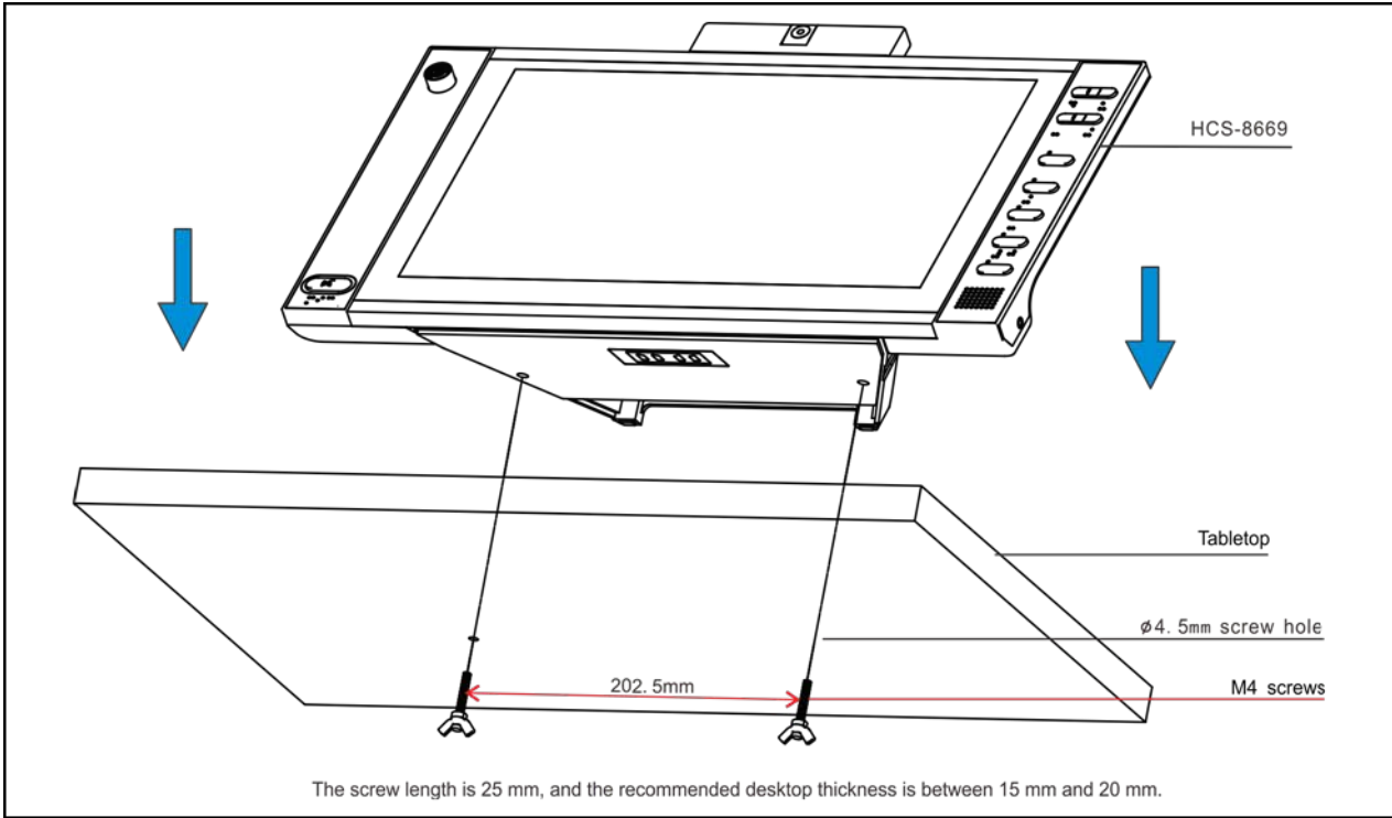
Figure: 3.2.5 Fixed installation of HCS-8669 series congress unit
