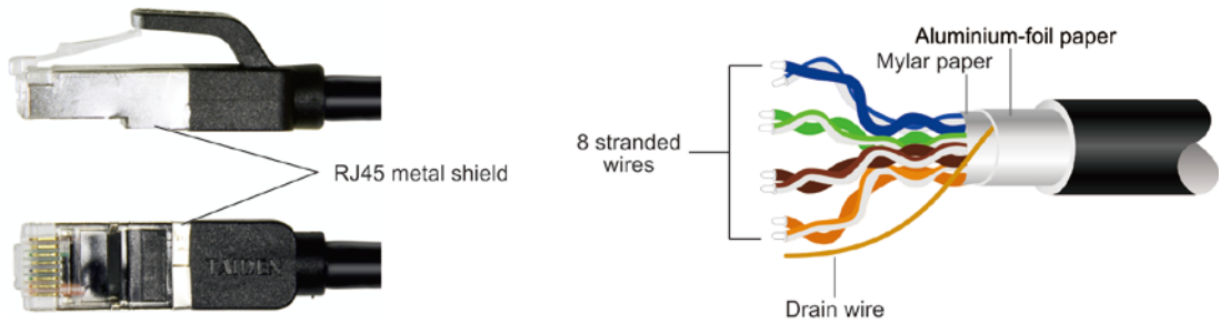
CAT5e cables as shown above, with a drain wire between aluminium-foil paper and mylar paper
