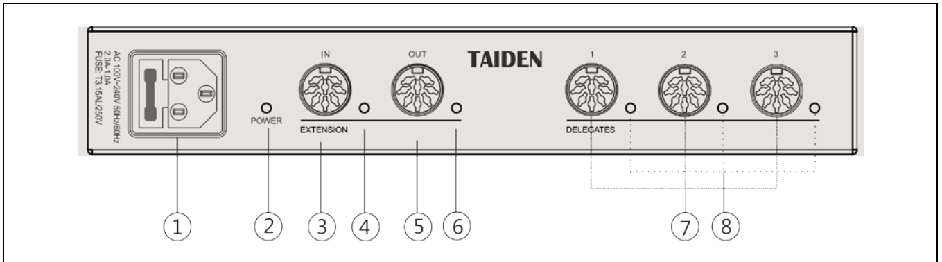
Figure 2.3.1 HCS-8600 series extension unit
