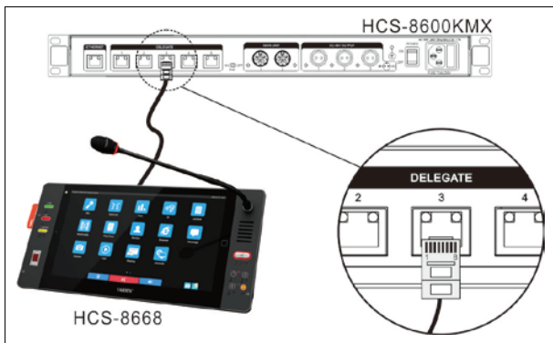
Figure 3.2.5 HCS-8638/8669/8668 series paperless multimedia congress terminal connecting to HCS-8600KMX Ethernet switcher (PoE)
