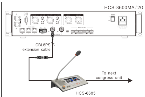
Figure 4.4 HCS-8685 Interpreter unit connected to the CMU or the EMU 2
