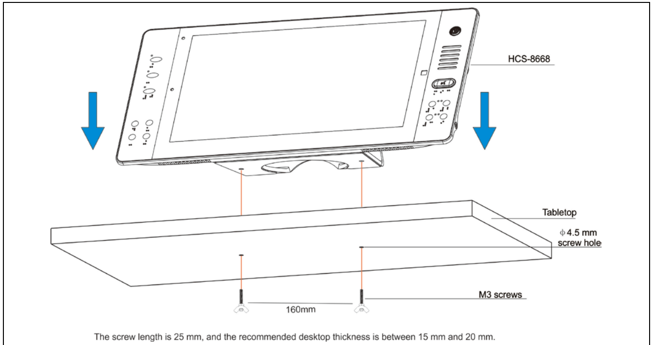
Figure 3.2.3 Fixed installation of HCS-8668/50 series congress unit
