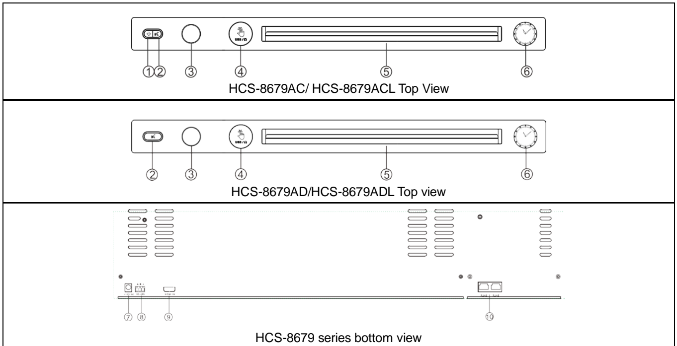
Figure 3.2.5 HCS-8679 series paperless multimedia congress terminal
