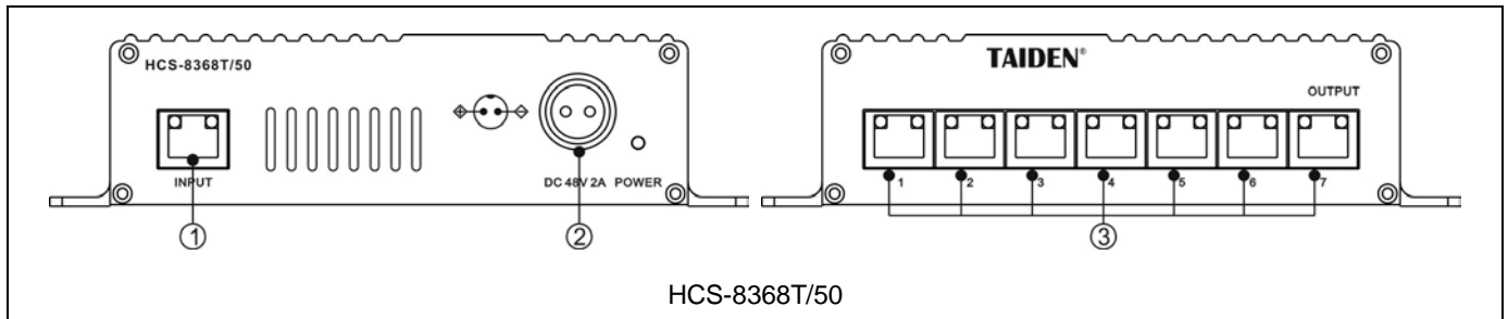
Figure 6.4.1 HCS-8368T Distributor
