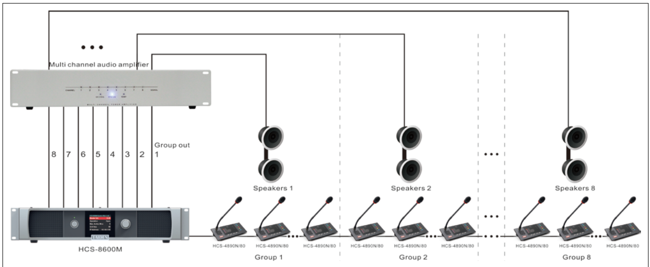
Figure 1.1.10 HCS-8600 Series Paperless Multimedia Congress System connected to a multi-channel audio amplifier with "N-1" function to cancel howl
