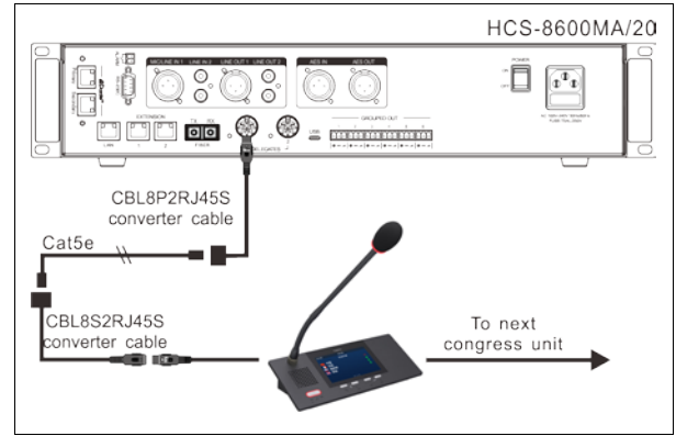
Figure 2.1.3 CMU connecting to contribution units (8P-DIN)2
