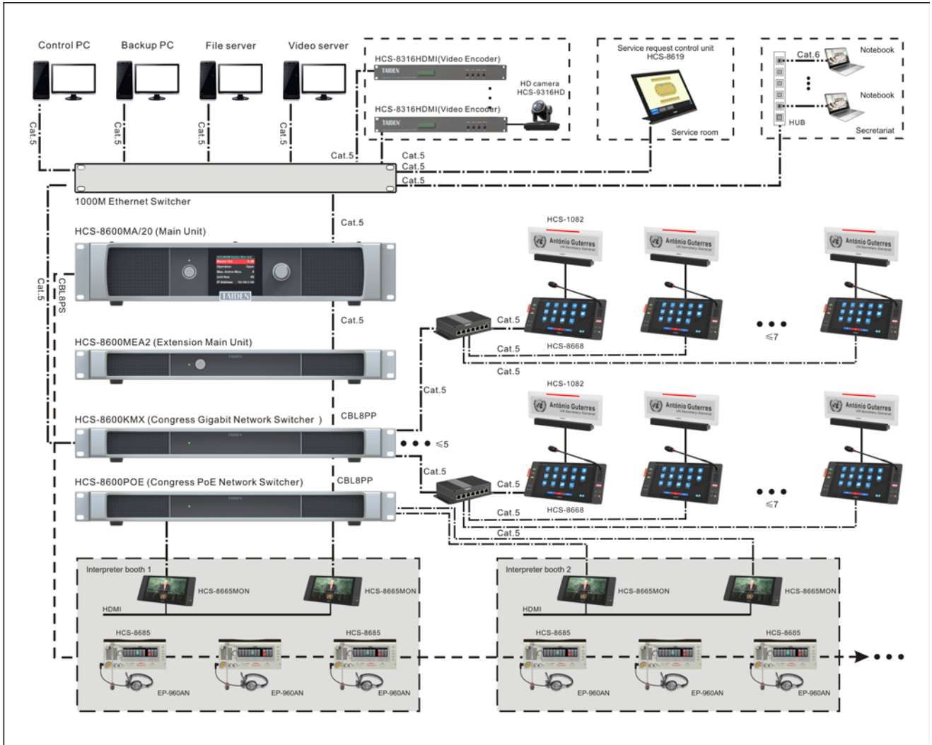
Figure 1.1.6 HCS-8668/50 Series Paperless Multimedia Congress System connection diagram (POE)
