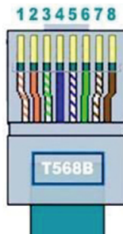
Wiring order (1-8) according to T568B standard: white-orange, orange, white-green, blue, white-blue, green, white-brown, brown
