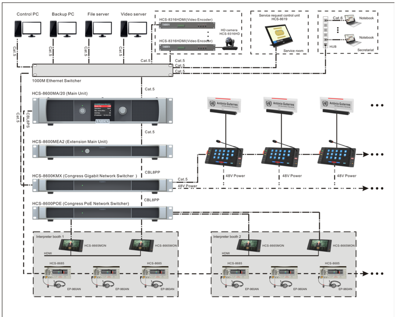
Figure 1.1.5 HCS-8668/50 Series Paperless Multimedia Congress System connection diagram
