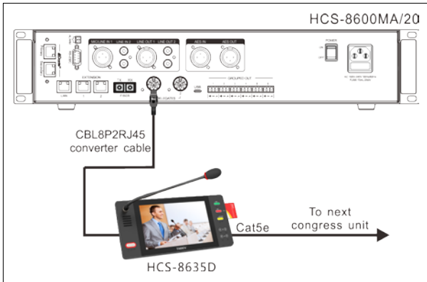
Figure 3.4.3 HCS-8635 series compact multimedia terminal connected to the CMU/EMU
