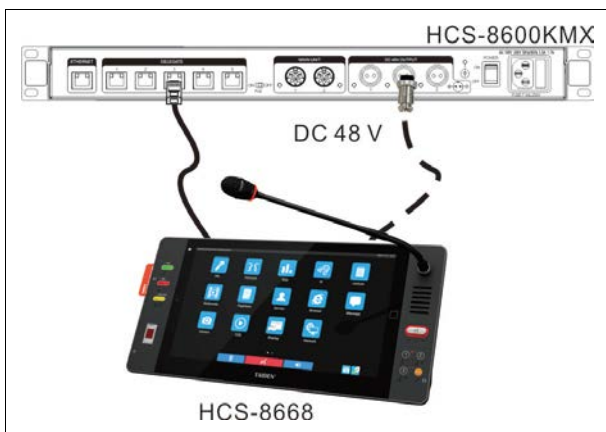
Figure 3.2.6 HCS-8638/8669/8668 series paperless multimedia congress terminal connecting to HCS-8600KMX Ethernet switcher (not PoE)
