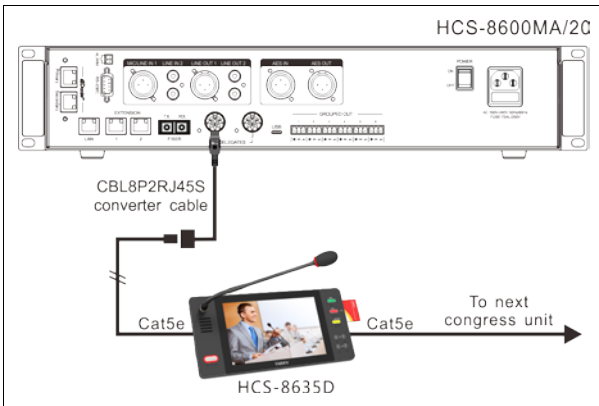
Figure 3.4.4 HCS-8635 series compact multimedia terminal connected to the CMU/EMU
