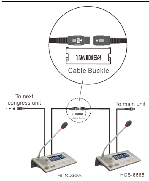
Figure 4.6 "Daisy-chain" connection between HCS-8685 Interpreter units
