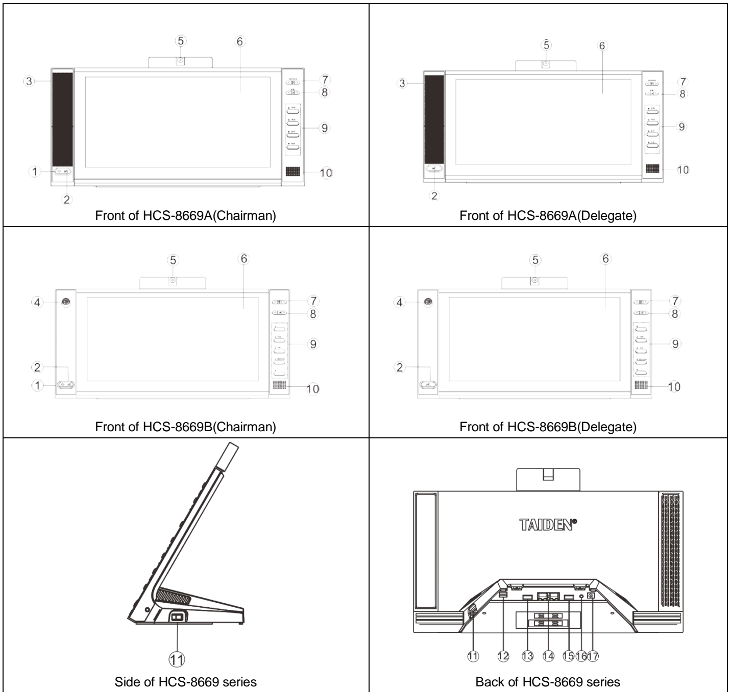
Figure 3.2.3 HCS-8669 series Paperless Multimedia Congress Terminal
