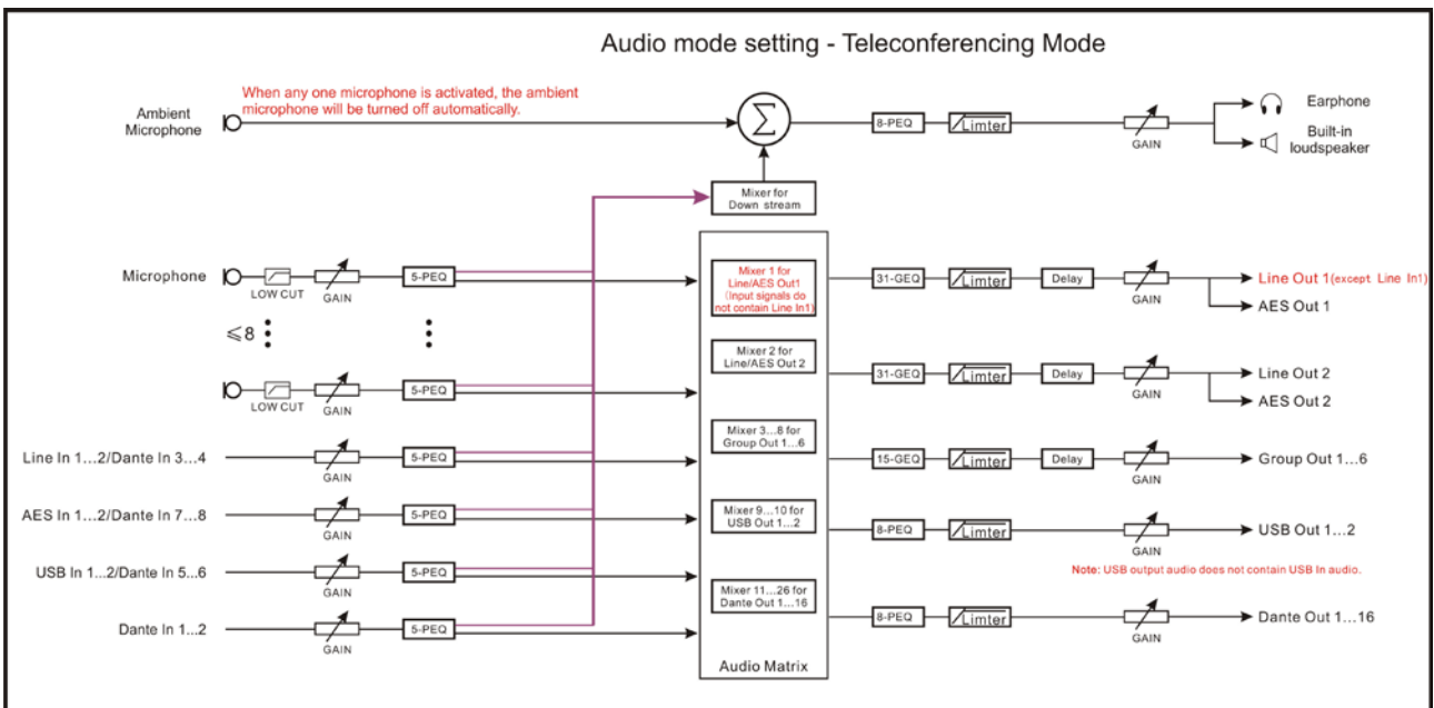
Figure 1.1.11 HCS-8600 series three modes of signal flow
