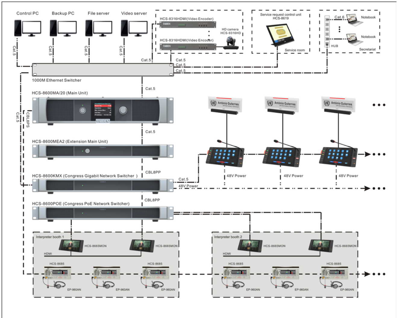
Figure 6.2.2 HCS-8668/50 Series Paperless Multimedia Congress System connection diagram
