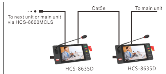
Figure 3.4.5 “Daisy-chain” connection between HCS-8635 series compact multimedia terminals
